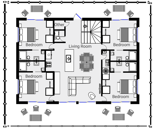
GROUPER HOUSE 2ND FLOOR
